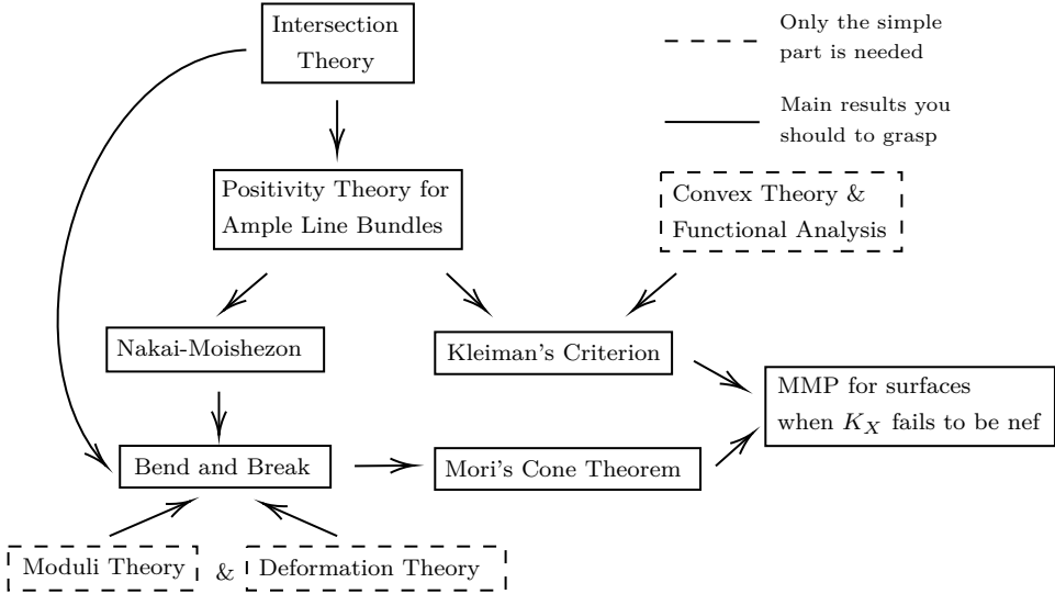
Figure 2.11.: Knowledge Framework
