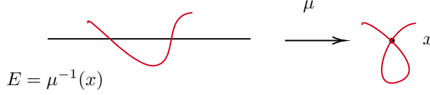
Figure 1.13.: strict transform
