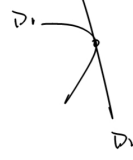
Figure 1.4.: Non-transversally
